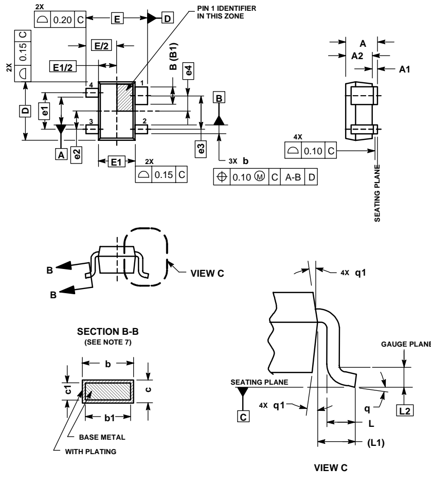
Figure 27. Outline Dimensions for SOT-343 (Case 318M-01, Issue 0)
