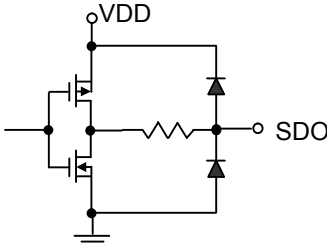
SDO terminal
