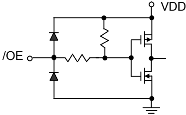
/OE terminal
