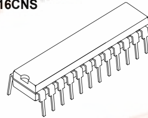
SDIP24-P-300-1.78
