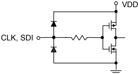
CLK, SDI terminal
