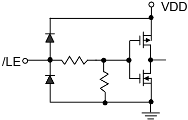
/LE terminal
