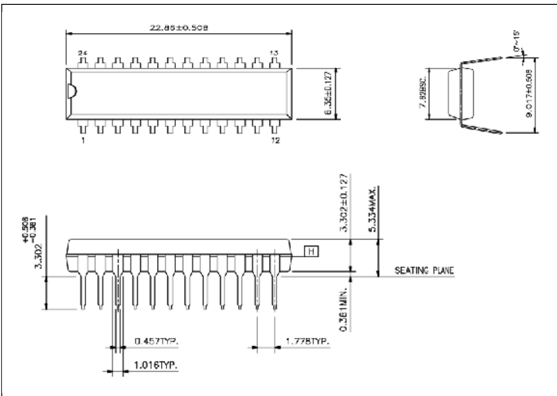
MBI5026CNS Outline Drawing
