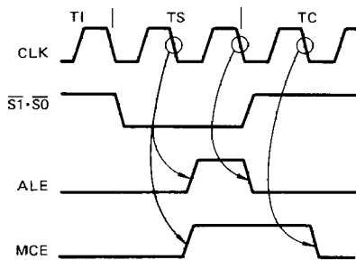
Fig. 11 — MCE OPERATION FOR AN INTA BUS CYCLE
