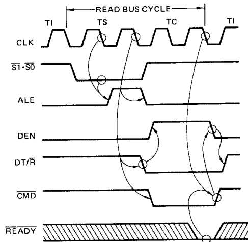
Fig. 6 – IDEL-READ-IDEL BUS CYCLES WITH MB = 0
