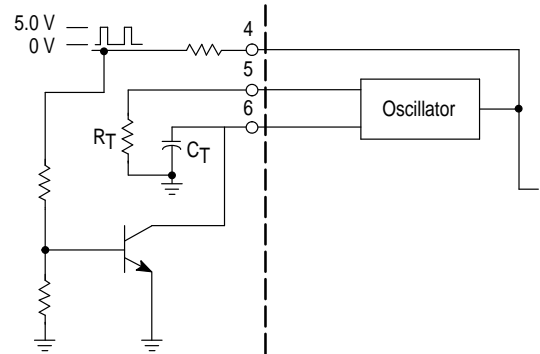
Figure 27. External Clock Synchronization
