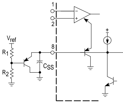
Figure 30. Buffered Maximum Clamp Level
