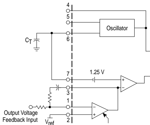
Figure 21. Voltage Mode Operation
