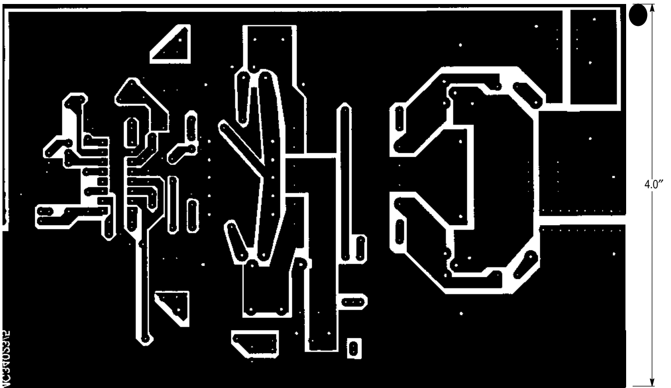
6.5" (Bottom View)
