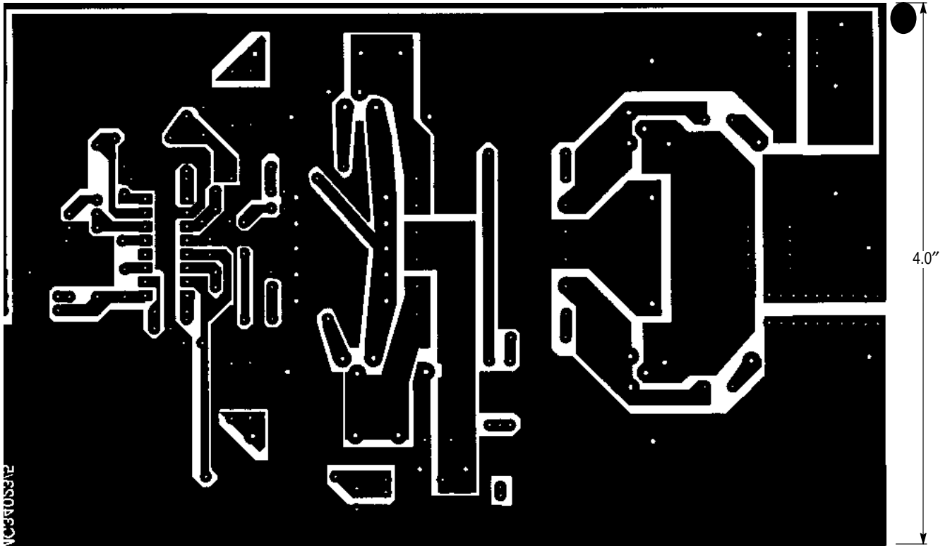
6.5" (Bottom View)
