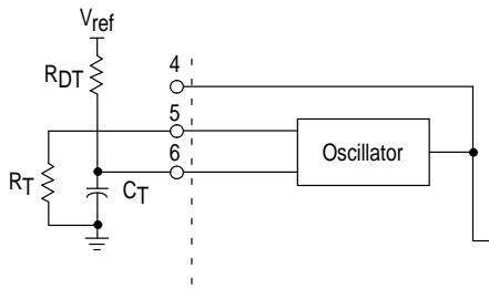
Figure 23. Dead Time Addition
