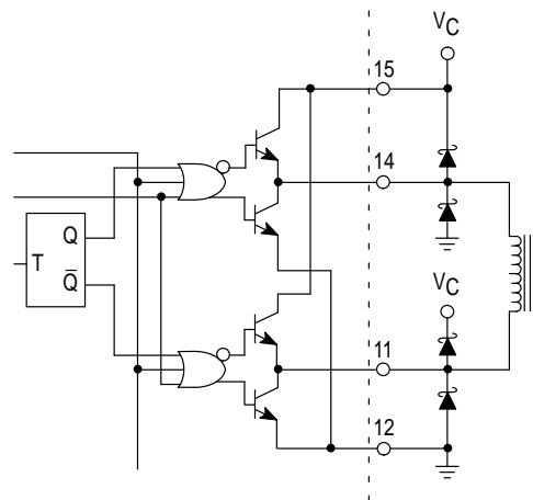
Figure 34. Direct Transformer Drive
