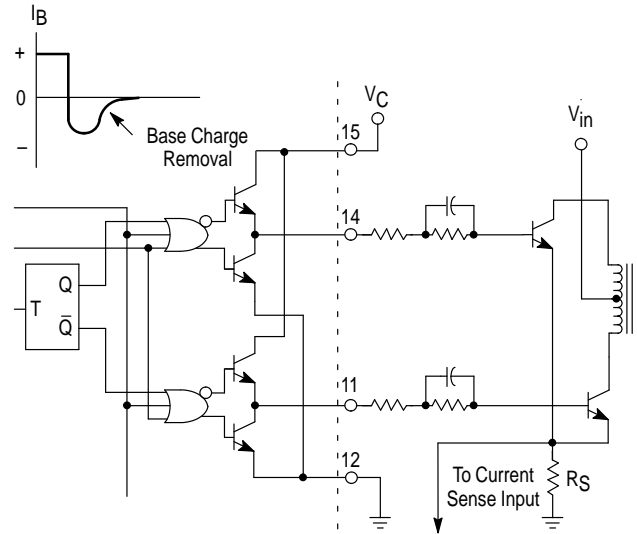
Figure 32. Bipolar Transistor Drive
