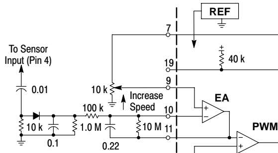
Figure 30. Controlled Acceleration/Deceleration
