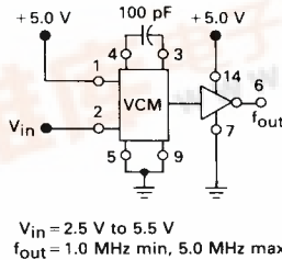
FIGURE 3 — VOLTAGE-CONTROLLED MULTIVIBRATOR
