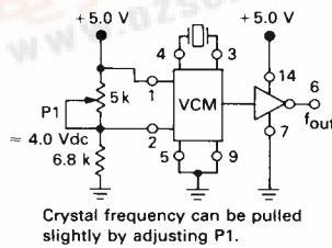
FIGURE 2 — CRYSTAL CONTROLLED MULTIVIBRATOR
