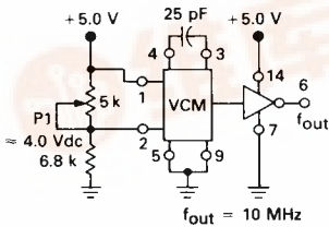
FIGURE 1 — ASTABLE MULTIVIBRATOR
