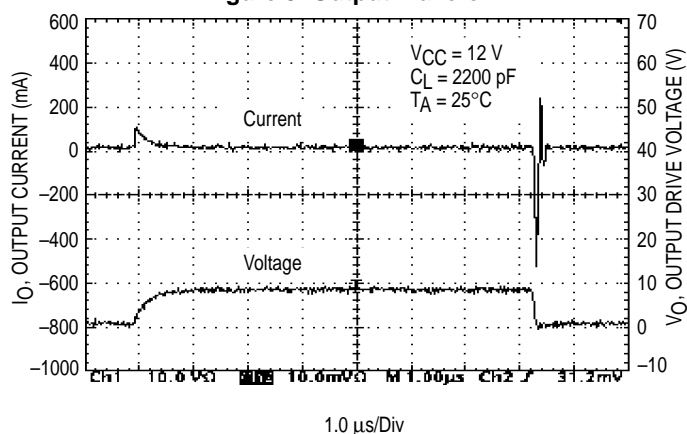
Figure 5. Output Waveform
