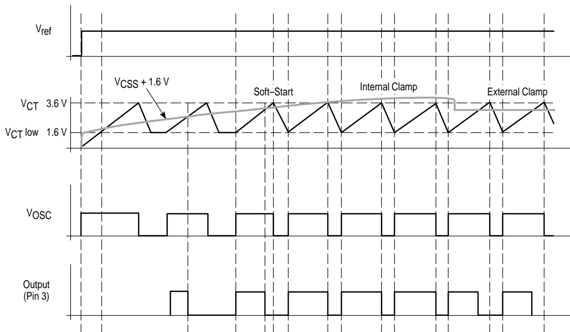
Figure 31. Soft-Start & Dmax
