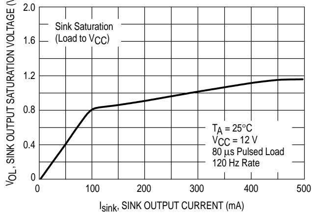
Figure 9. Sink Output Saturation Voltage versus Sink Current
