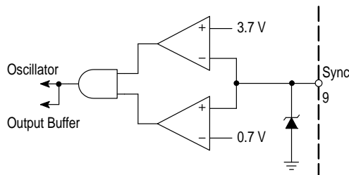
Figure 36. Synchronization
