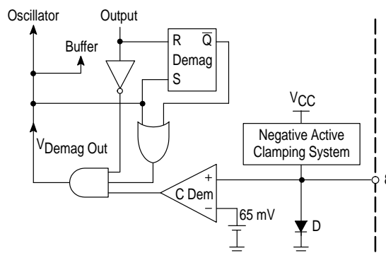
Figure 38. Demagnetization Block
