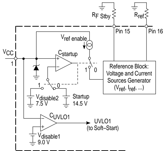
Figure 47. V_{CC} Management
