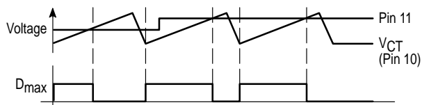
Figure 43. Maximum Duty Cycle Control
