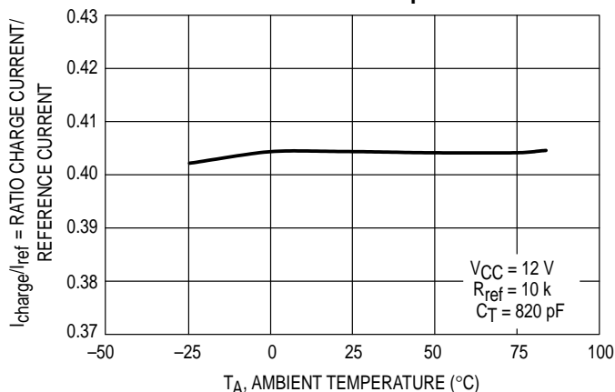
Figure 4. Ratio Charge Current/Reference Current versus Temperature
