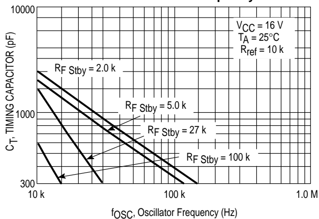
Figure 2. Standby Mode Timing Capacitor versus Oscillator Frequency
