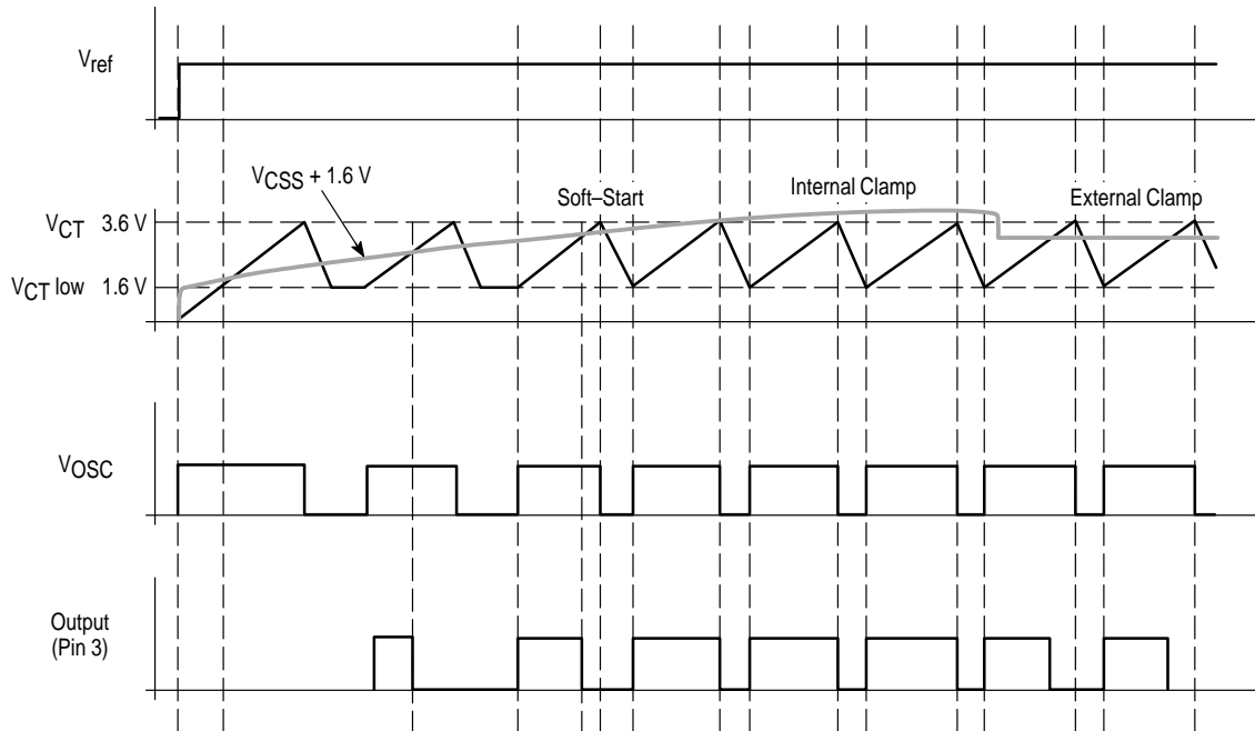
Figure 31. Soft-Start & Dmax
