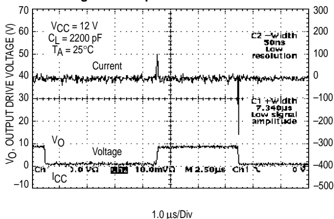
Figure 6. Output Cross Conduction
