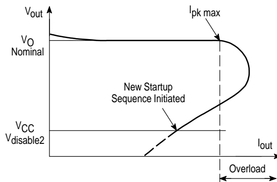
Figure 45. Foldback Characteristic
