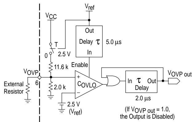
Figure 46. Overvoltage Protection
