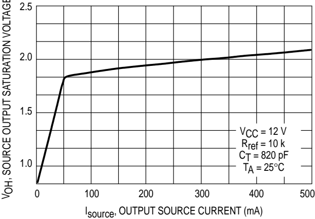
Figure 8. Source Output Saturation Voltage versus Load Current
