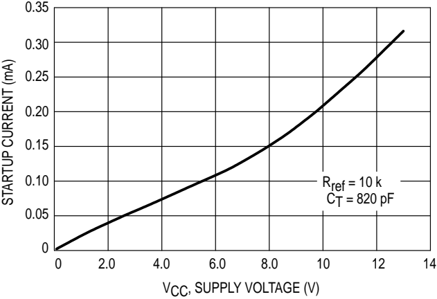
Figure 16. Startup Current versus V CC
