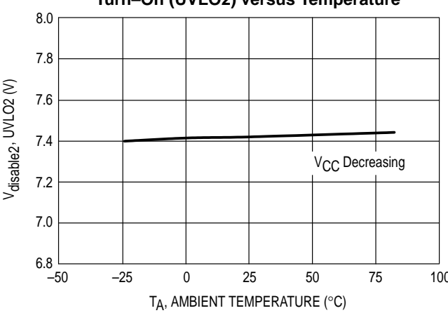
Figure 21. Disable Voltage After Threshold Turn-On (UVLO2) versus Temperature
