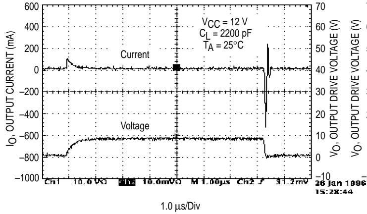
Figure 5. Output Waveform
