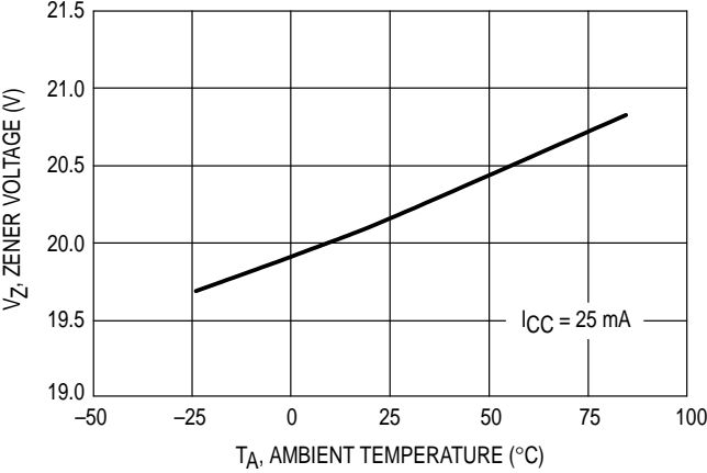
Figure 18. Power Supply Zener Voltage versus Temperature
