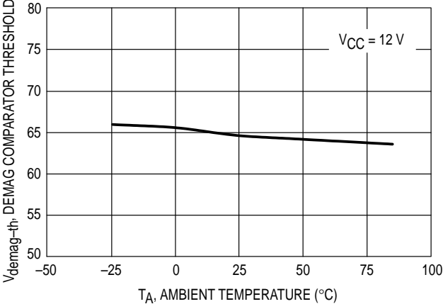
Figure 12. Demag Comparator Threshold versus Temperature
