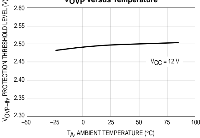
Figure 22. Protection Threshold Level on V_{\text{OVP}} versus Temperature
