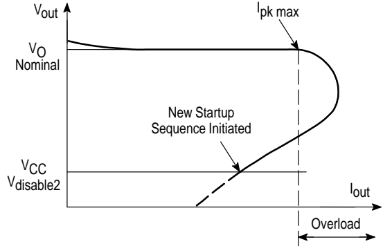
Figure 45. Foldback Characteristic
