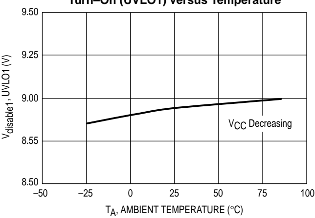
Figure 20. Disable Voltage After Threshold Turn-On (UVLO1) versus Temperature
