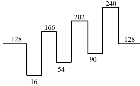
Digital Cb-input code(16~240) 525/60 and 625/50 system 100%amplitude,100%saturation color bar
