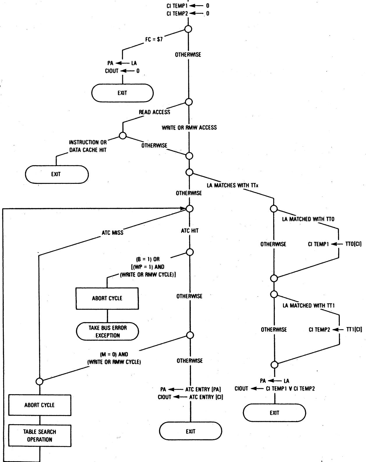
Figure 9-8. Address Translation General Flowchart
