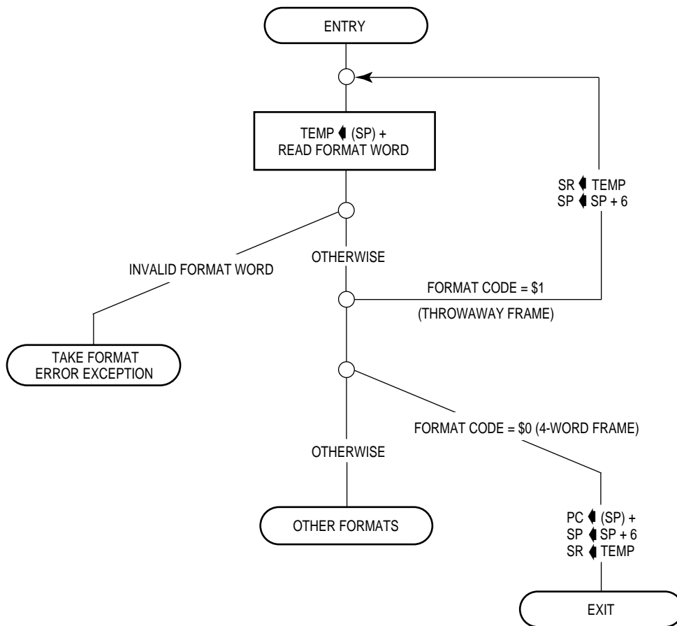
Figure 8-8. RTE Instruction for Throwing Four-Word Frame
