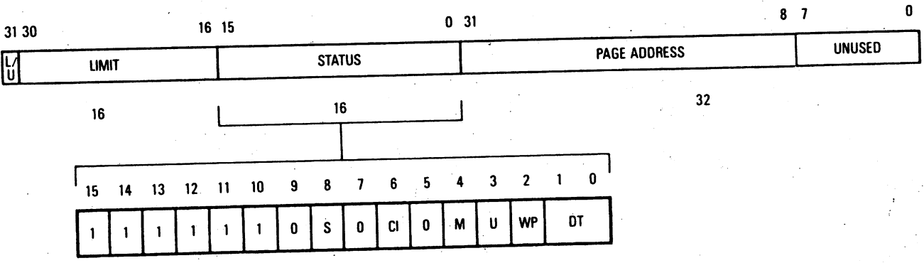
Figure 9-13. Long-Format Early Termination Page Descriptor
