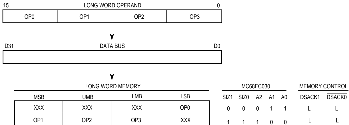
Figure 7-15. Misaligned Long-Word Transfer to Long-Word Port
