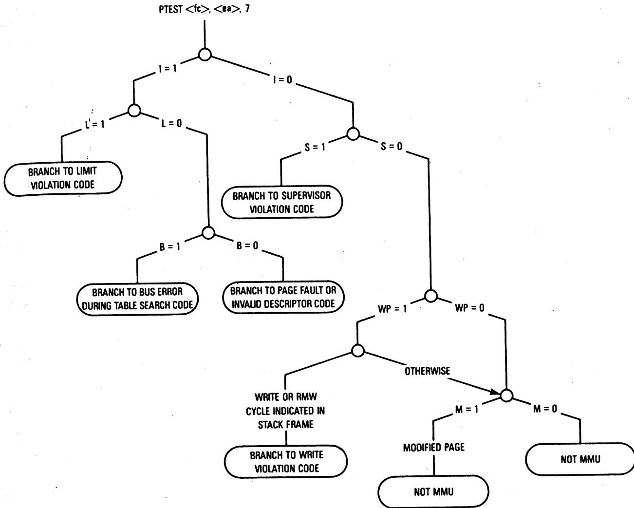
Figure 9-40. MMU Status Interpretation PTEST Level 7
