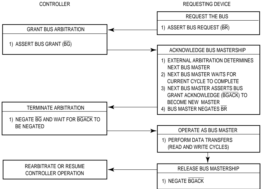
Figure 7-59. Bus Arbitration Flowchart for Single Request
