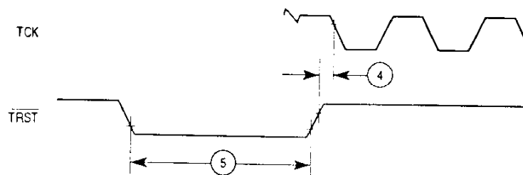
Figure 6-9. \overline{\text{TRST}} Timing Diagram
