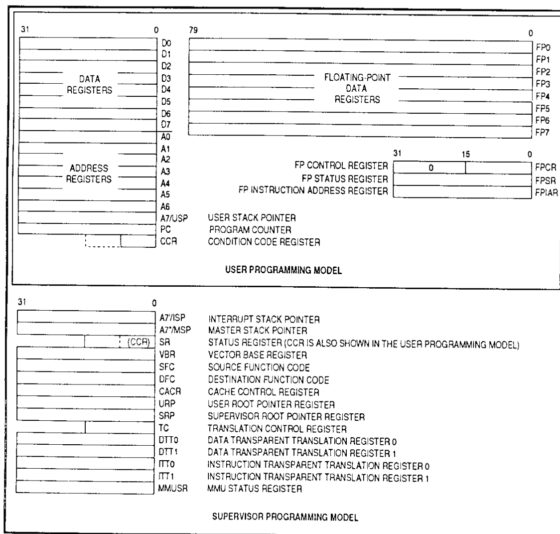
Figure 1-2. Programming Model
