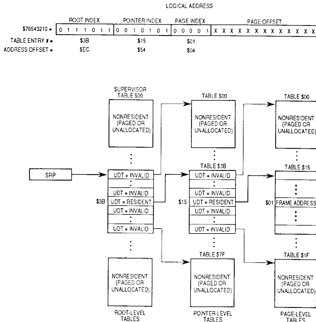
Figure 3-16. Translation Table with Nonresident Tables
