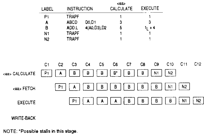
Figure 10-3. Interlocked Stages
