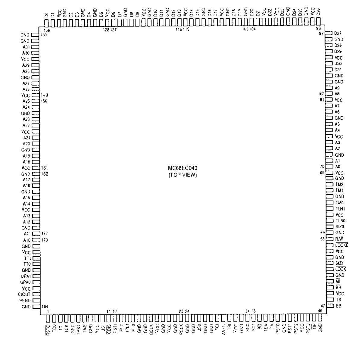
MC68EC040 184 Pin QFP Pin Assignment
