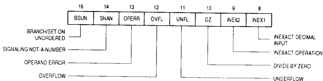
Figure 9-5. FPSR Exception Status Byte
