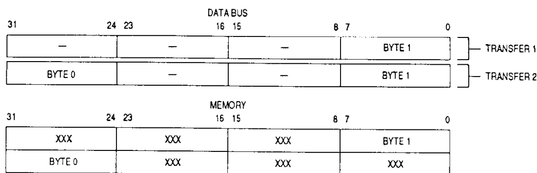
Figure 7-6. Example of a Misaligned Word Transfer
