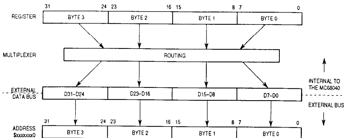
Figure 7-3. Data Multiplexing
