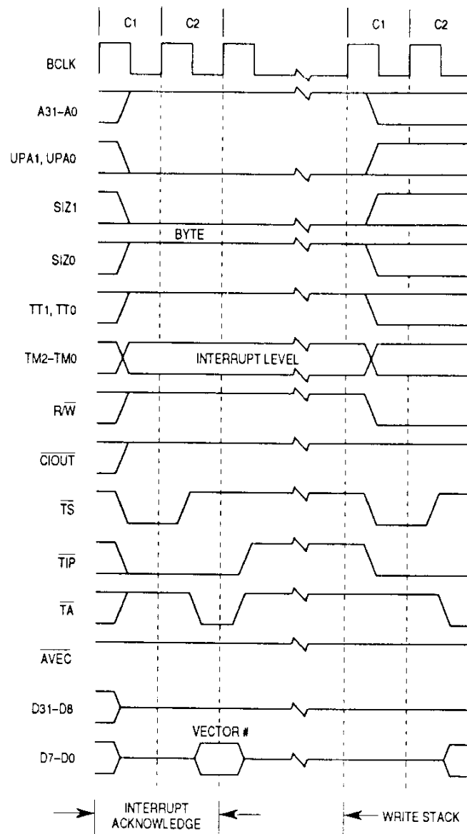
Figure 7-22. Interrupt Acknowledge Bus Cycle Timing
