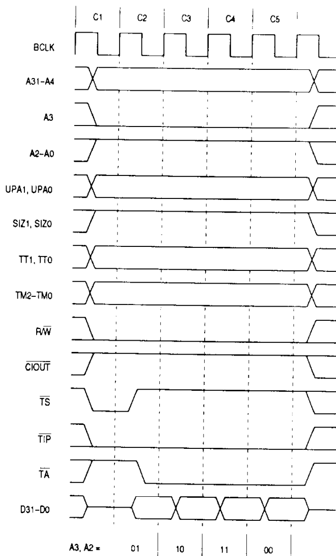
Figure 7-17. Line Write Transfer Timing
