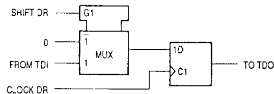
Figure 6-2. Bypass Register
