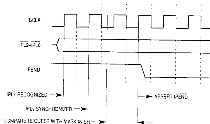
Figure 7-20. Assertion of \overline{\text{IPEND}}
