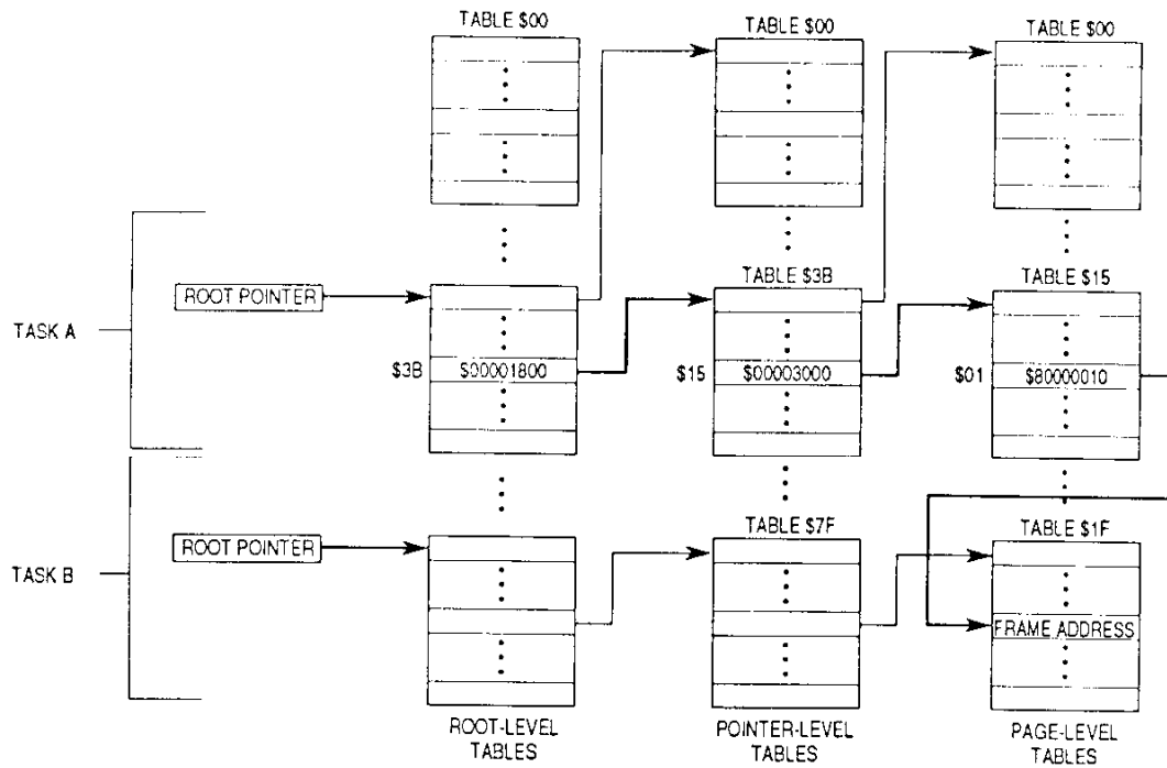
Figure 3-14. Translation Table Using Indirect Descriptors
