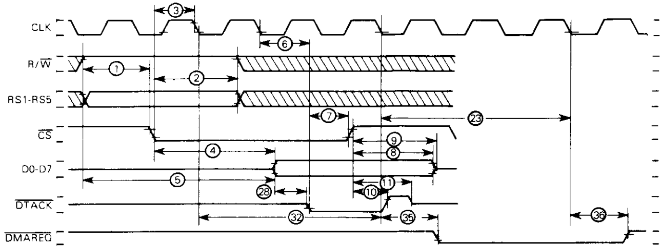
Figure 6-2. Read Cycle Timing Diagram
