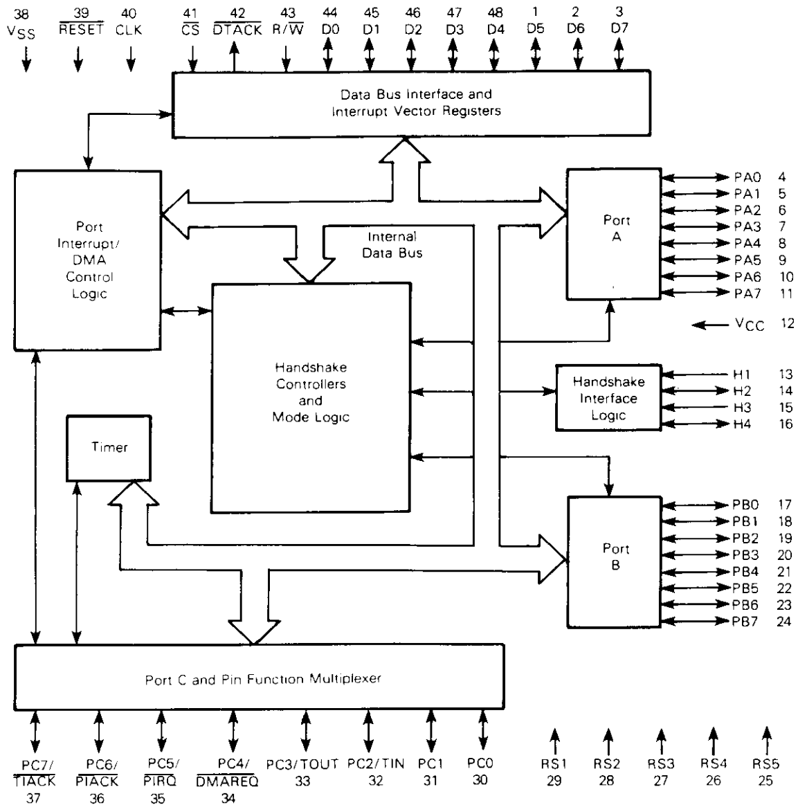
Figure 1-1. Block Diagram
