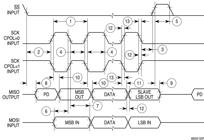
Figure A-19 QSPI Timing — Slave, CPHA = 1
