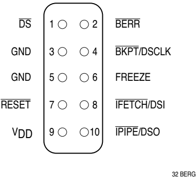
Figure 5-11 BDM Connector Pinout
