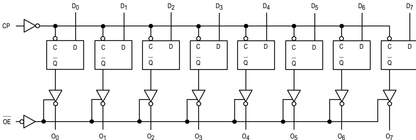
LOGIC DIAGRAM
