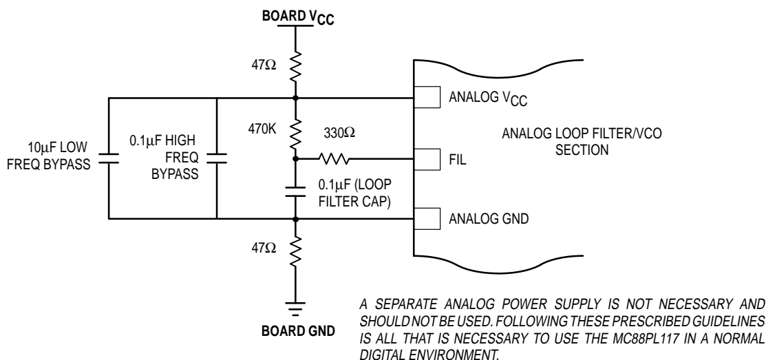
Figure 12. Recommended Loop Filter and Analog Isolation Scheme
