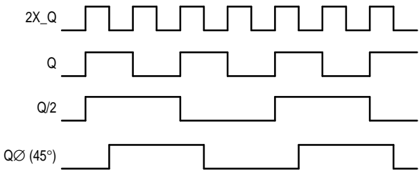
Figure 10. 88PL117 Output Waveforms
