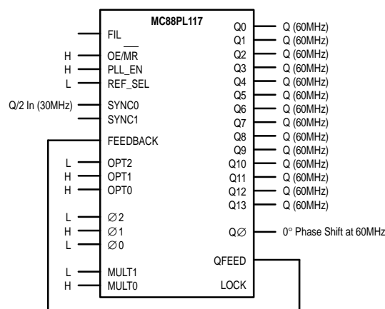
Figure 4. Output Frequency Configuration 4 (OPT0 = H, OPT1 = H, OPT2 = L Q/2 Input Frequency, MULT0 = H, MULT1 = L)
