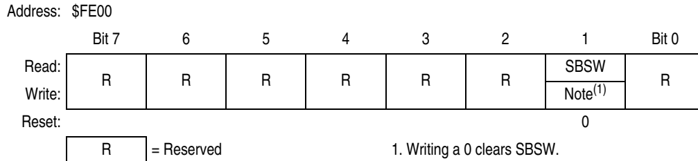
Figure 19-7. SIM Break Status Register (SBSR)
