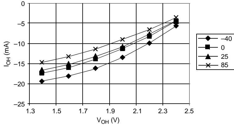
Figure 20-6. Typical High-Side Driver Characteristics – Port PTC4–PTC0 ( V_{DD} = 2.7 \text{ Vdc} )
