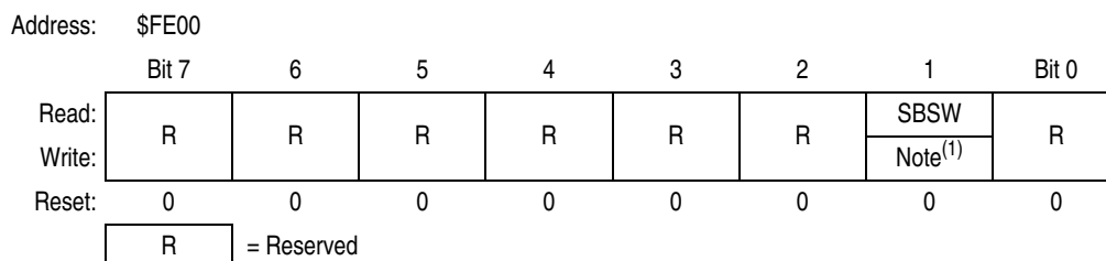
Figure 15-20. SIM Break Status Register (SBSR)
