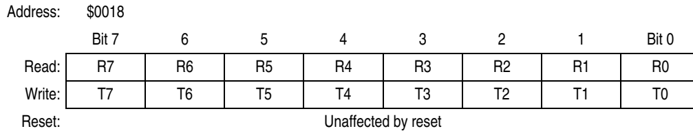
Figure 14-16. ESCI Data Register (SCDR)
