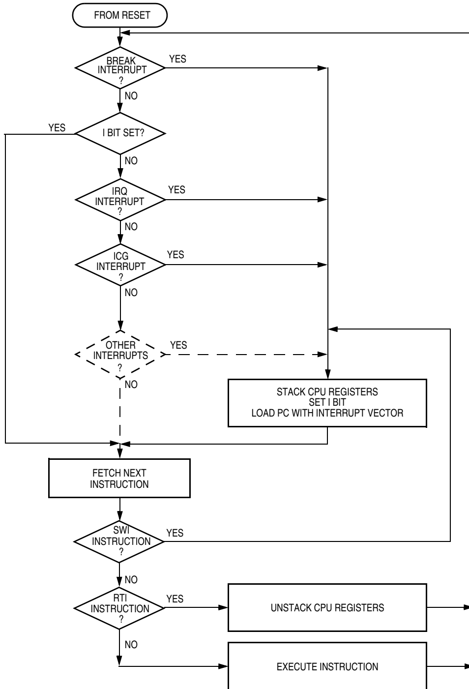
Figure 13-6. Interrupt Processing
