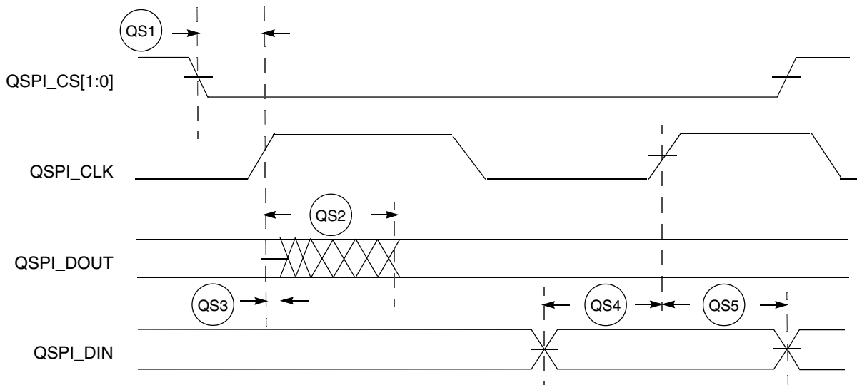
Figure 19. QSPI Timing
