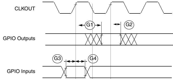
Figure 12. GPIO Timing
