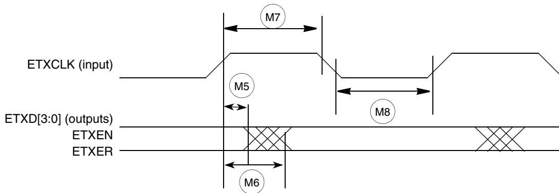
Figure 16. MII Transmit Signal Timing Diagram
