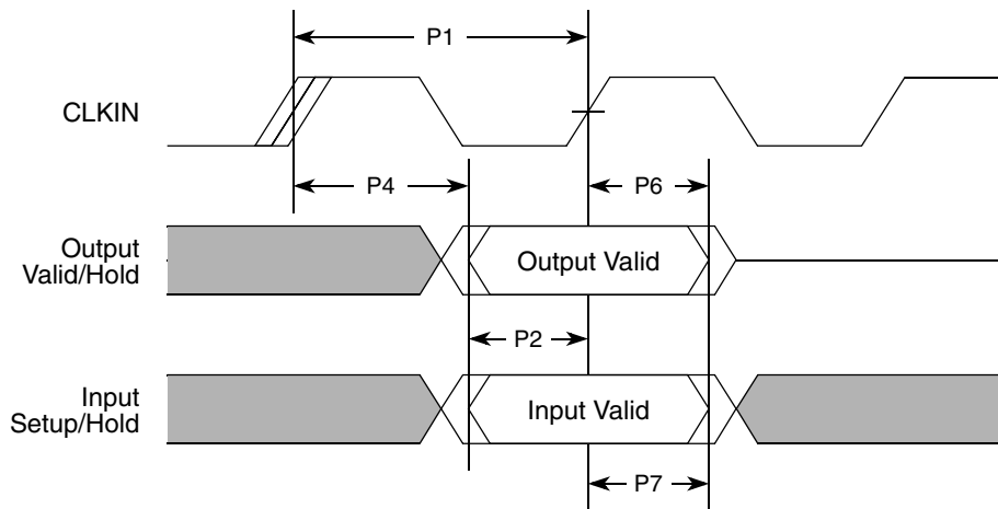
Figure 14. PCI Timing
