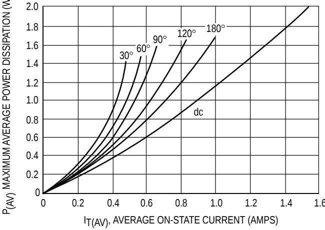
FIGURE 8 — POWER DISSIPATION
