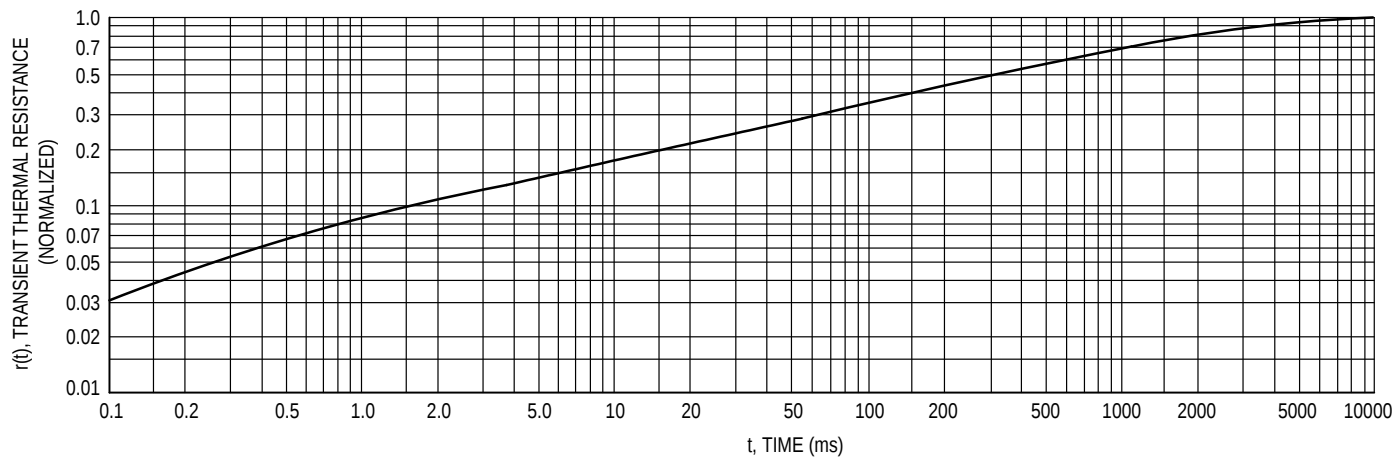
FIGURE 4 — THERMAL RESPONSE
