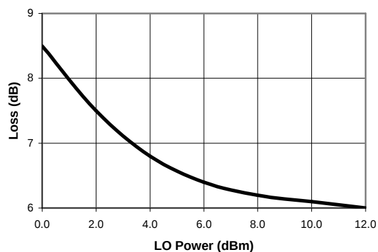
Conversion Loss vs. LO Power (RF @ 1000 MHz—10 dBm, IF = 50 MHz)
