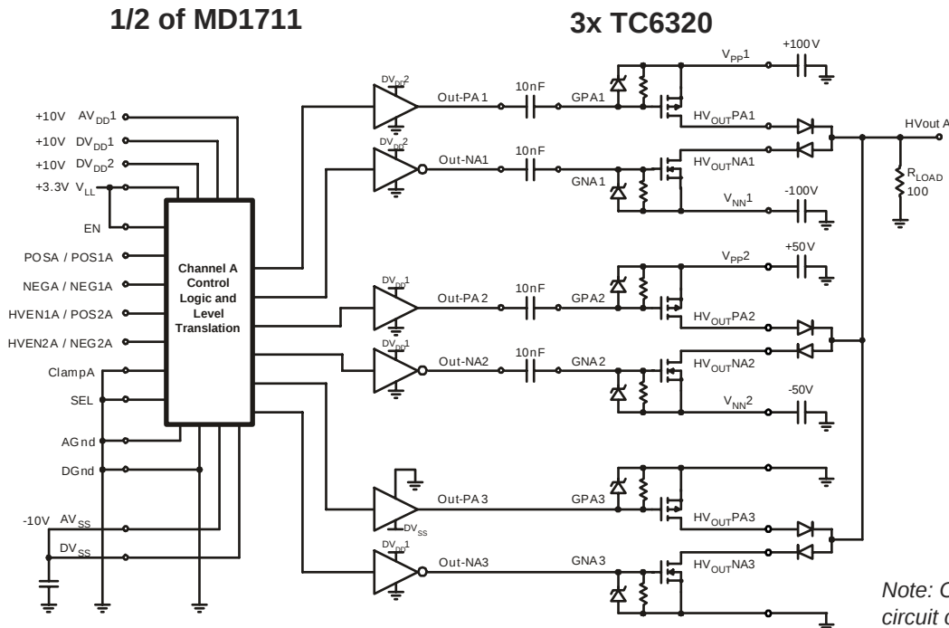
Test Circuit for Channel A
