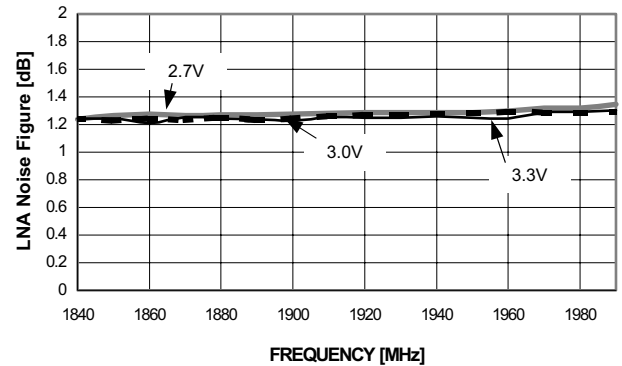
LNA Noise Figure vs. V_{DD} @ 25°C, V_{DD} = 2.7V, 3.0V, 3.3V
