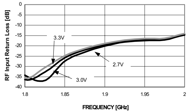
Downconverter RF Input Return Loss vs. V DD @ 25°C, V DD = 3.2V, 3.0V, 3.3V V CTRL = 3.0V
