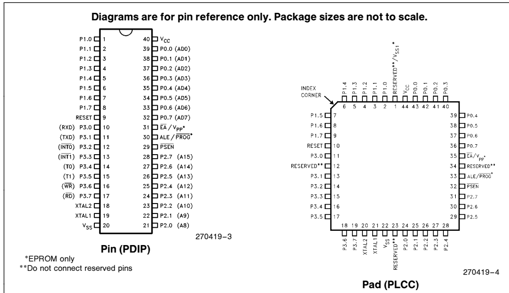
Figure 3. Pin Connections
