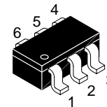
SC-74 CASE 318F STYLE 8
