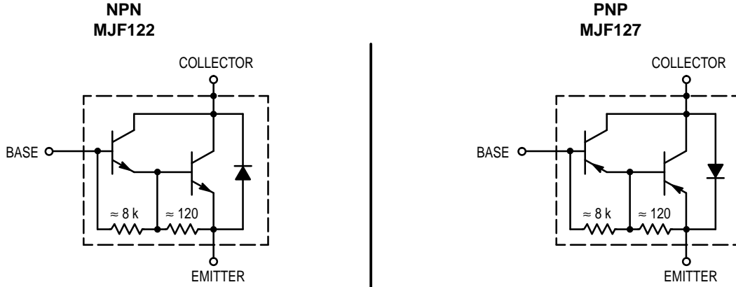
Figure 13. Darlingon Schematic
