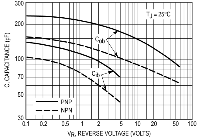
Figure 7. Typical Capacitance
