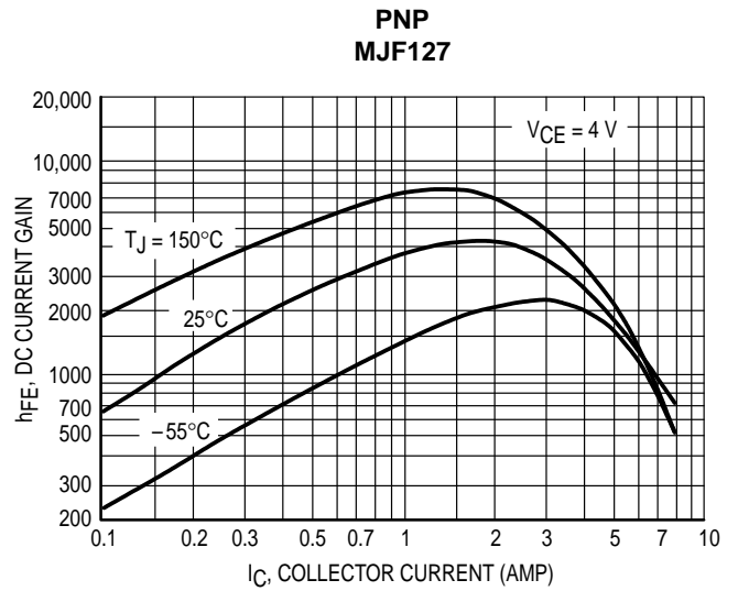
Figure 8. Typical DC Current Gain
