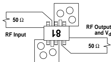
Figure 13. RF Layout.
