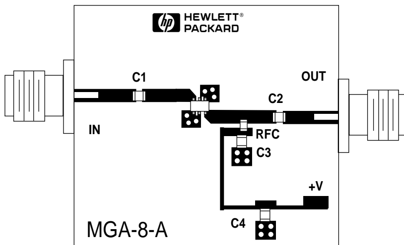
Figure 16. Complete Application Circuit.
