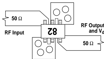
Figure 13. RF Layout.
