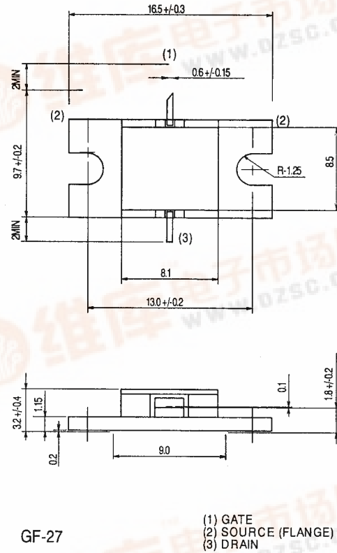
OUTLINE DRAWING Unit : millimeters
