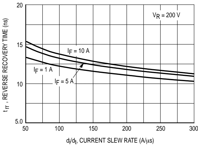
Figure 7. Typical t_{rr} Characteristics, T J = 25°C
