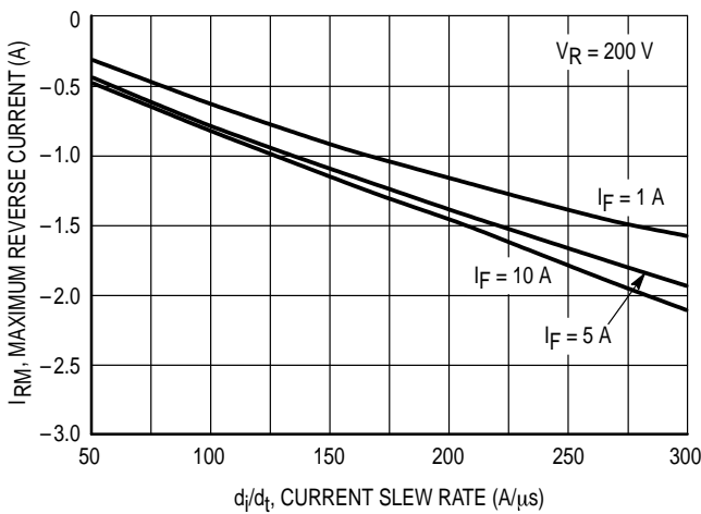
Figure 9. Typical I RM Characteristics, T J = 25°C
