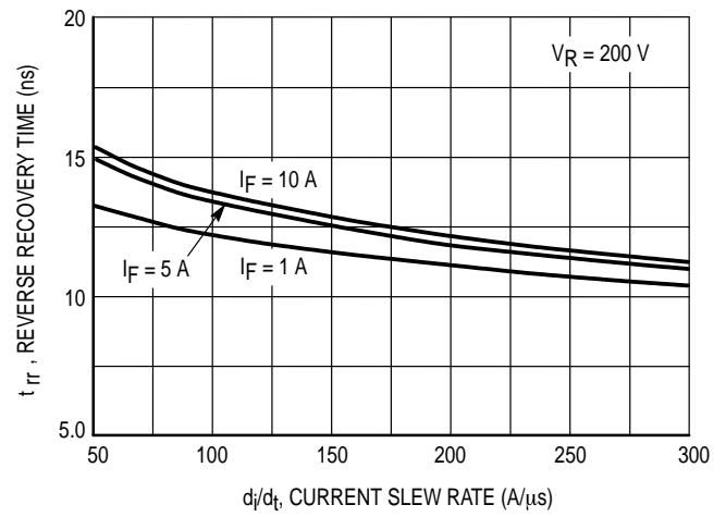
Figure 8. Typical t_{rr} Characteristics, T J = 125°C
