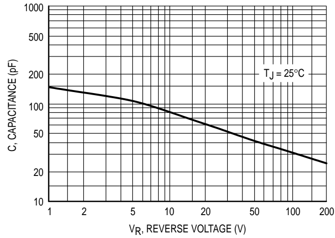
Figure 12. Typical Capacitance
