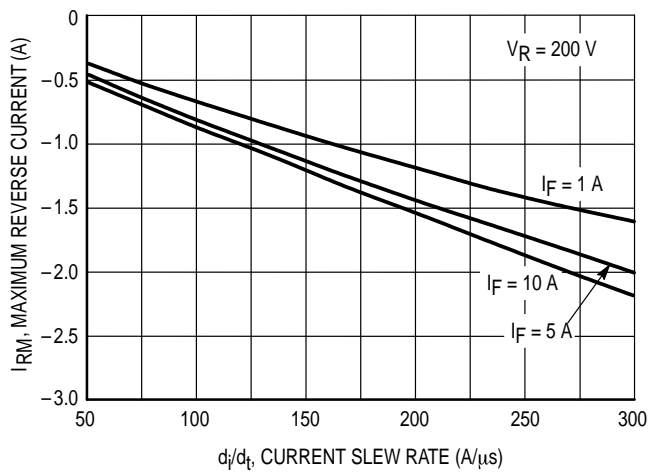
Figure 10. Typical I RM Characteristics, T J = 125°C
