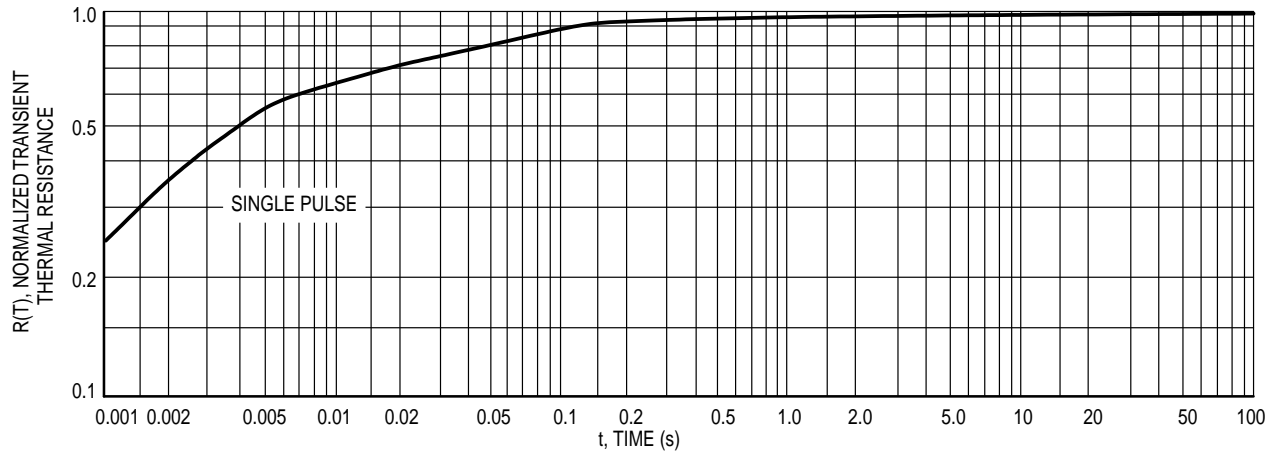
Figure 11. Typical Thermal Response
