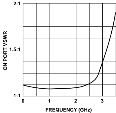
Figure 4. On Port VSWR vs. Frequency. V_{\text{Control}} = -5 \text{ V.}
