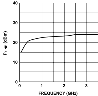
Figure 5. Output Power vs. Frequency. V_{\text{Control}} = -7 \text{ V.}
