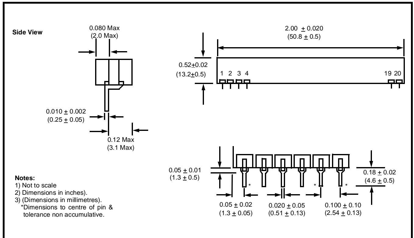
Figure 9 -Mechanical Data
