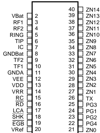
Figure 2 - Pin Connections
