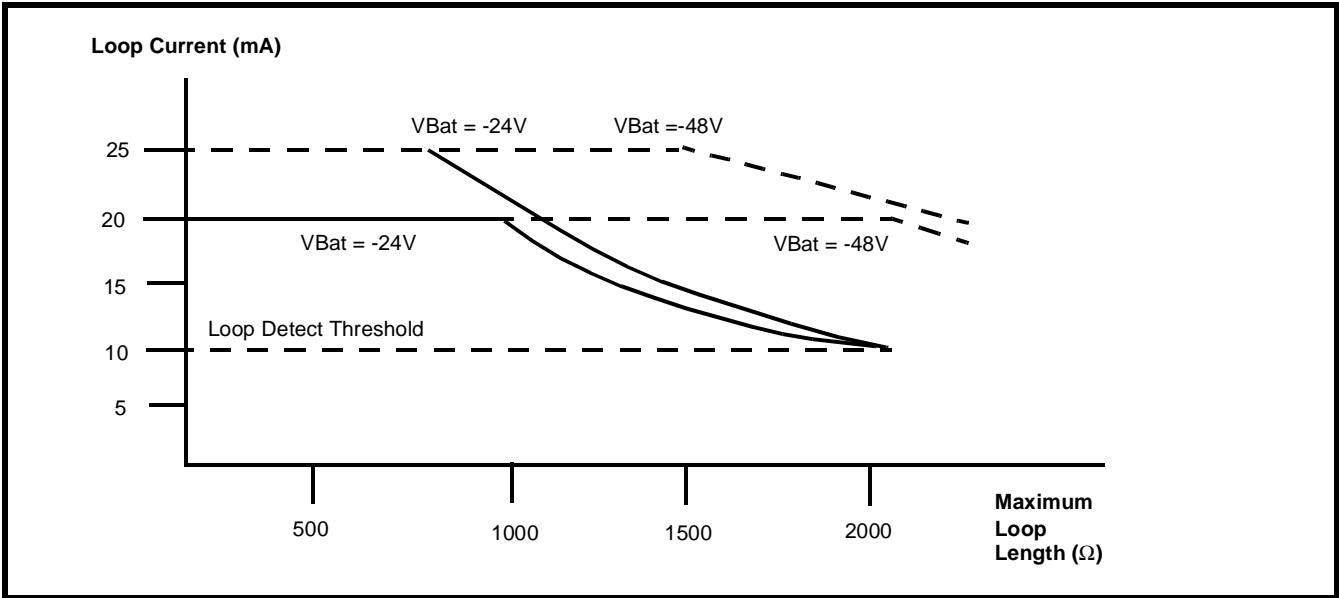
Figure 3a - Loop Current vs. Maximum Loop Current
