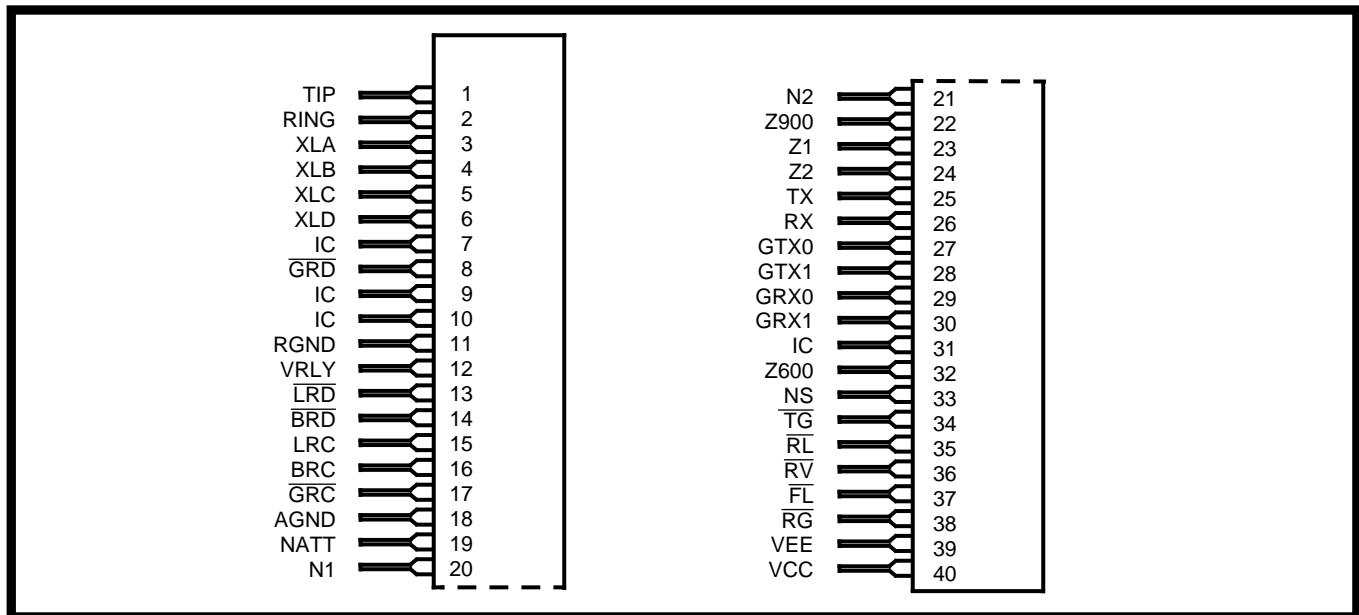
Figure 2 - Pin Connections
