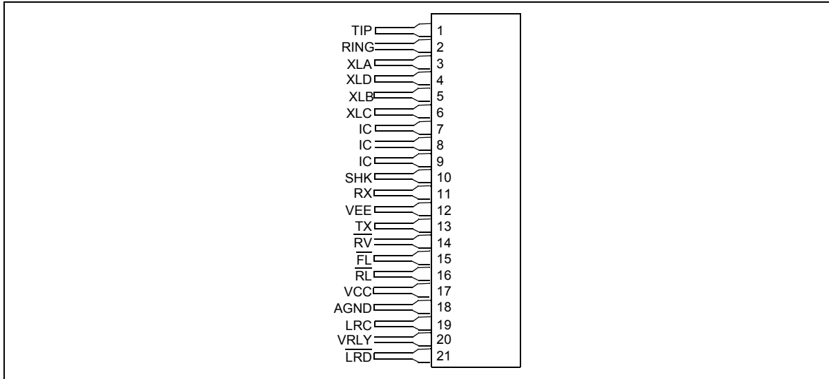
Figure 2 - Pin Connections
