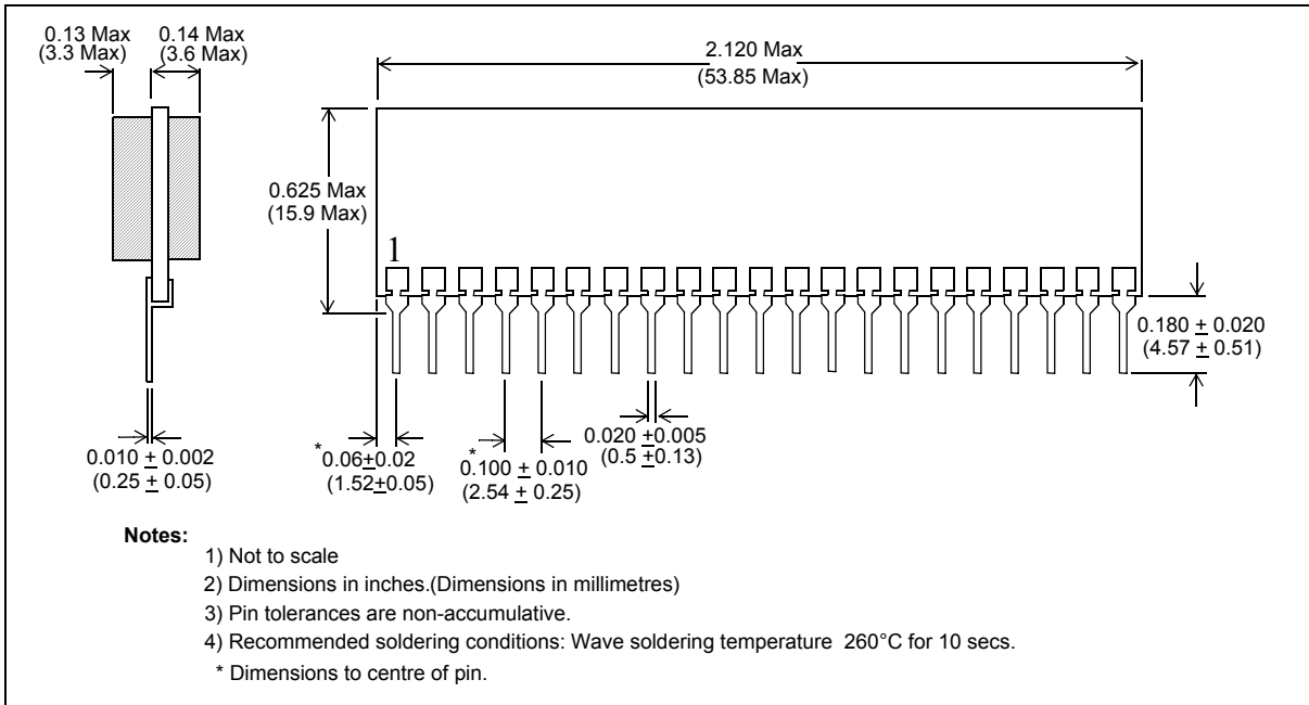
Figure 9 - Mechanical Data
