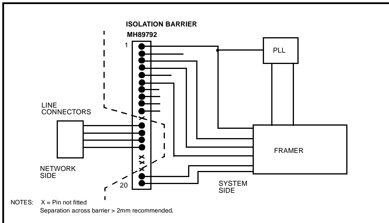
Figure 3c - Application Circuit
