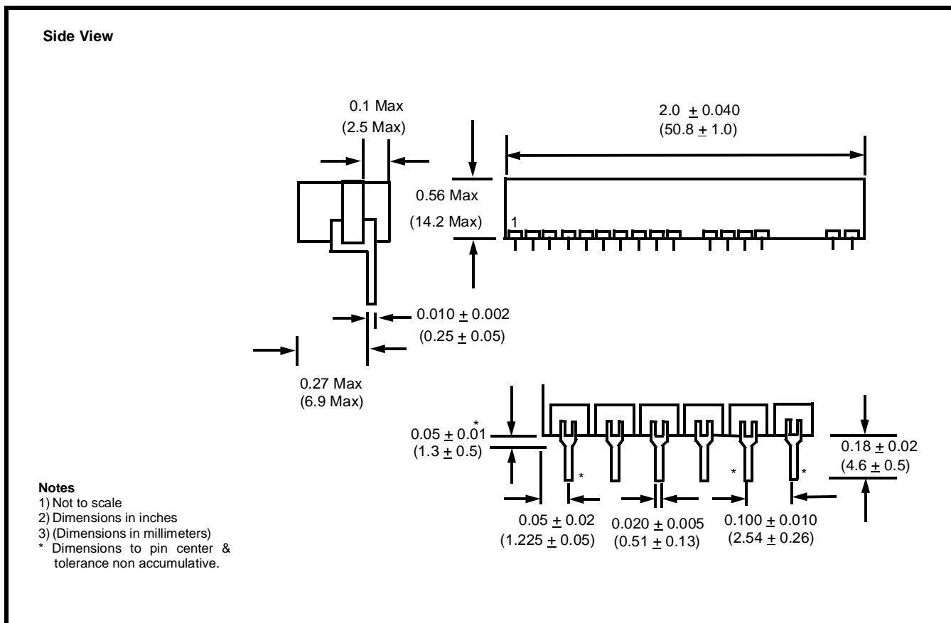
Figure 4 - Mechanical Data
