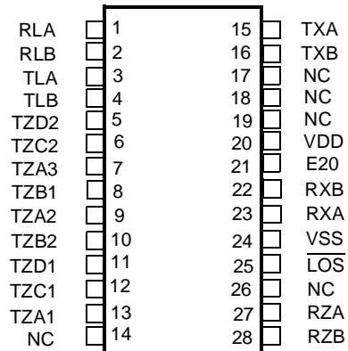
Figure 2 - Pin Connections
