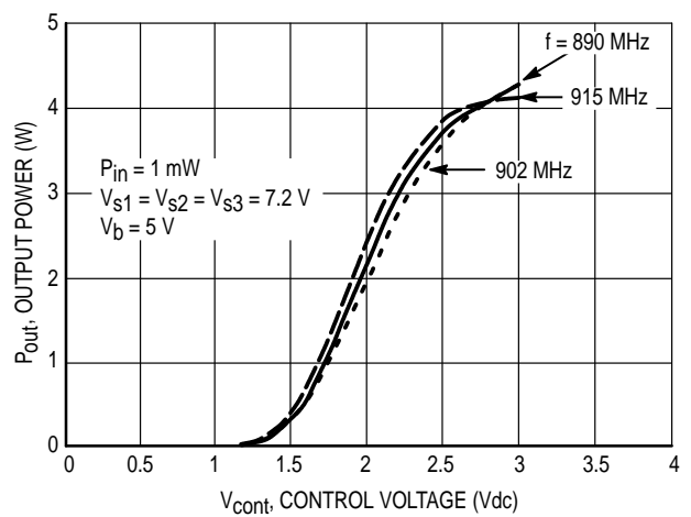
Figure 4. Output Power versus Control Voltage
