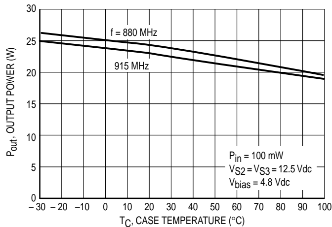
Figure 6. Output Power versus Case Temperature for Maximum Input Power
