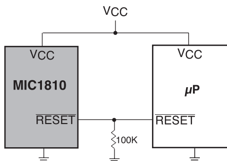
Figure 3. \overline{\text{RESET}} Valid to V_{CC} = 0V
