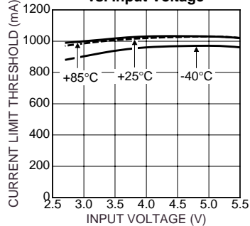
Current-Limit Threshold vs. Input Voltage
