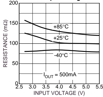
On-Resistance vs. Input Voltage
