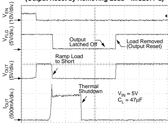
Thermal Shutdown (Output Reset by Removing Load—MIC2077-2)
