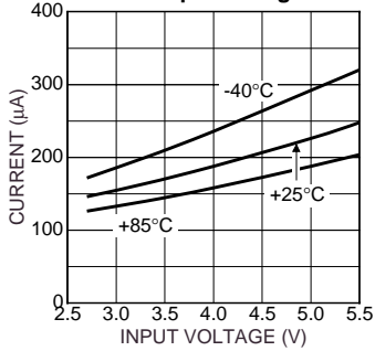
Supply On-Current vs. Input Voltage
