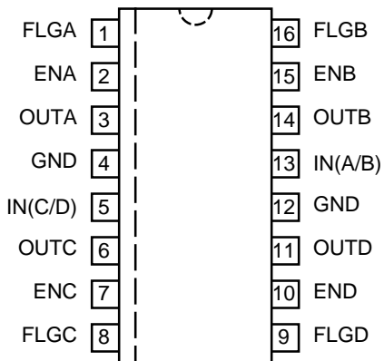
16-Lead SOP (M) 16-Lead Wide SOP (WM)
