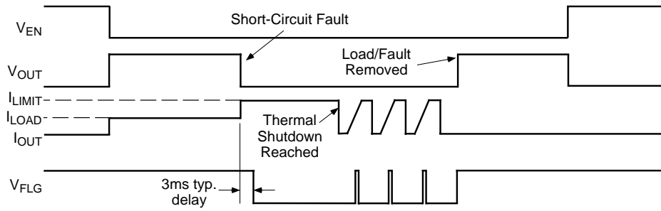
Figure 2. MIC2077-2 Fault Timing
