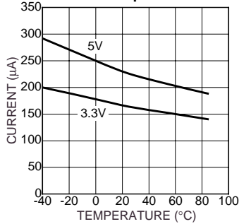
Supply On-Current vs. Temperature
