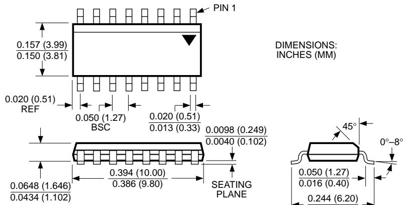
16-Lead SOP (M)
