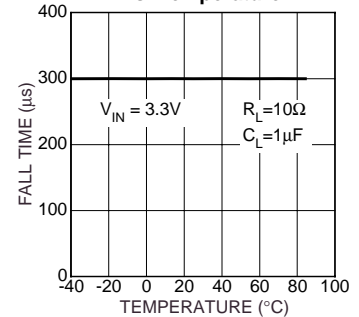
Fall Time vs. Temperature
