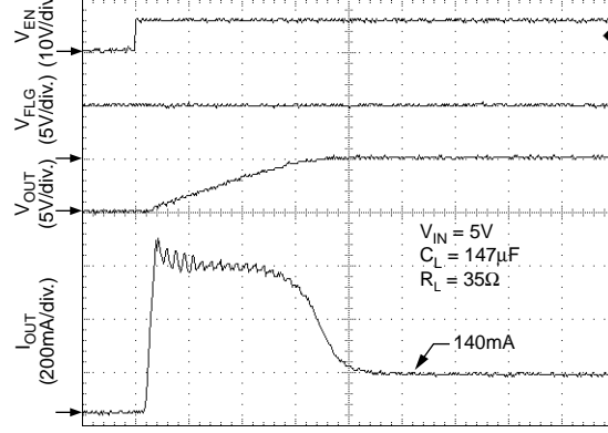
Turn-On (MIC2027-1)
