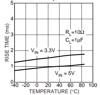
Turn-On Rise Time vs. Temperature
