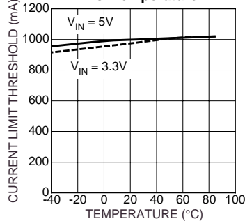
Current-Limit Threshold vs. Temperature
