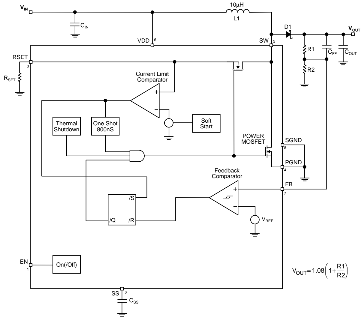
Figure 1. Block Diagram
