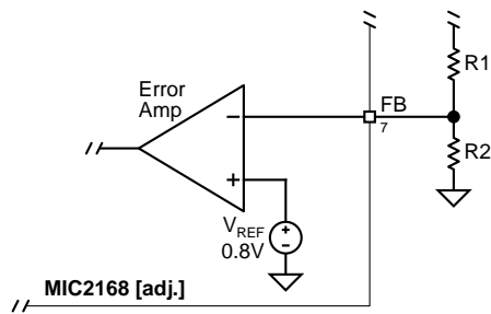
Figure 2. Voltage-Divider Configuration
