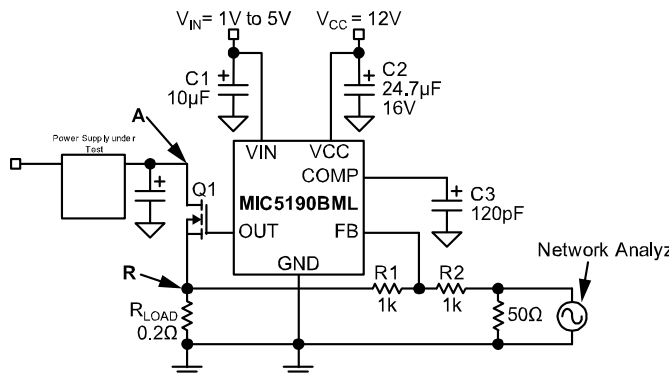
Figure 9. Output Impedance Measurement
