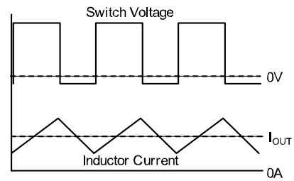
Figure 2. Continuous Operation
