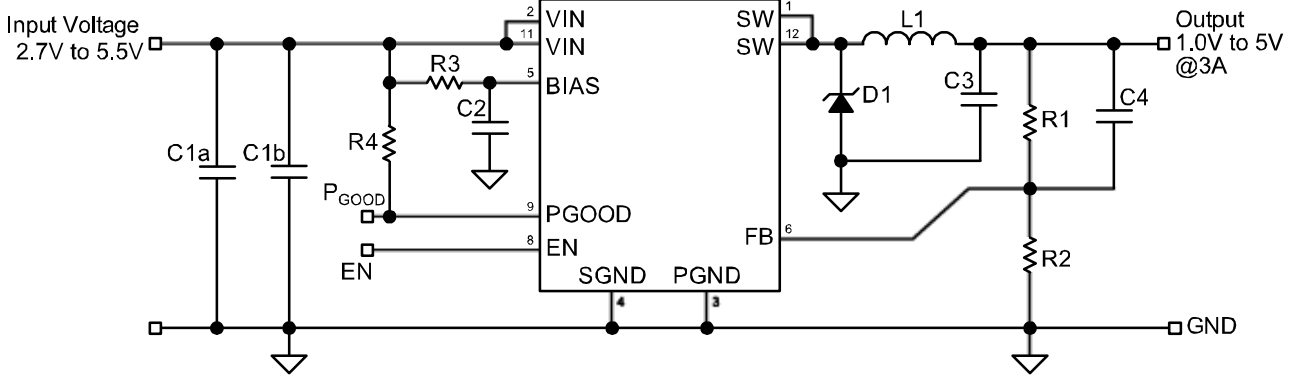
MIC2207 Schematic
