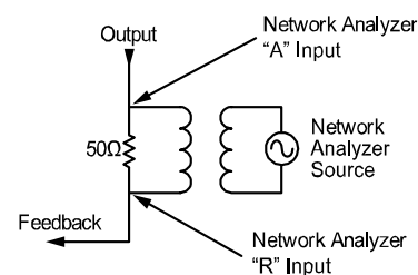
Figure 7. Transformer Injection
