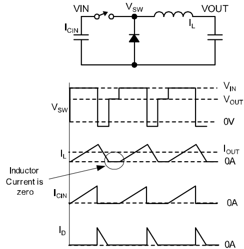
Figure 5. Discontinuous Operation
