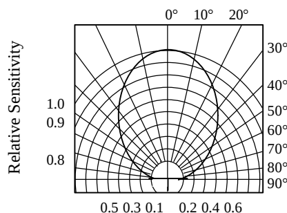
FIG.5 SENSITIVITY DIAGRAM
