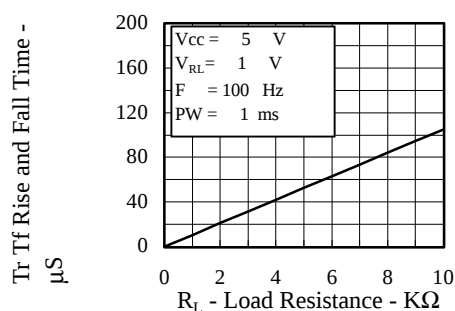
FIG.3 RISE AND FALL TIME VS LOAD RESISTANCE
