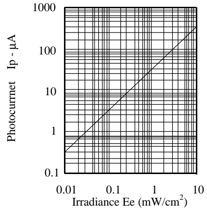
FIG.6 PHOTOCURRENT VS. IRRADIANCE = 850 nm
