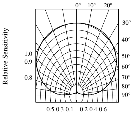
FIG.7 SENSITIVITY DIAGRAM
