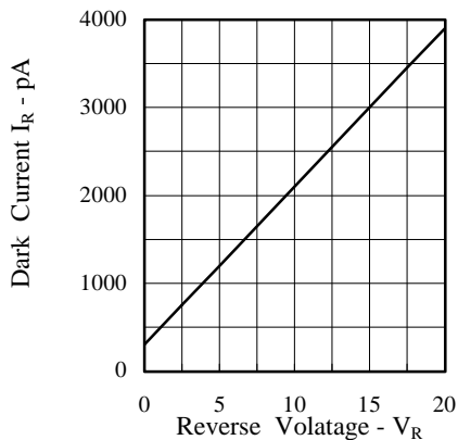
FIG.1 DARK CURRENT VS REVERSE VOLTAGE TEMP= 25^{\circ}\text{C} , E_e=0\text{ mW/cm}^2
